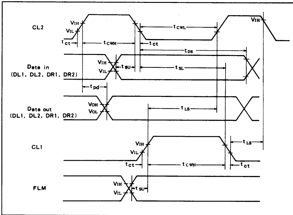
Figure 1 Timing Waveform
