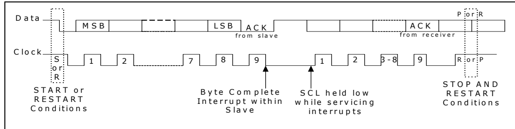
Figure 35. Data Transfer on the I 2 C* Bus
