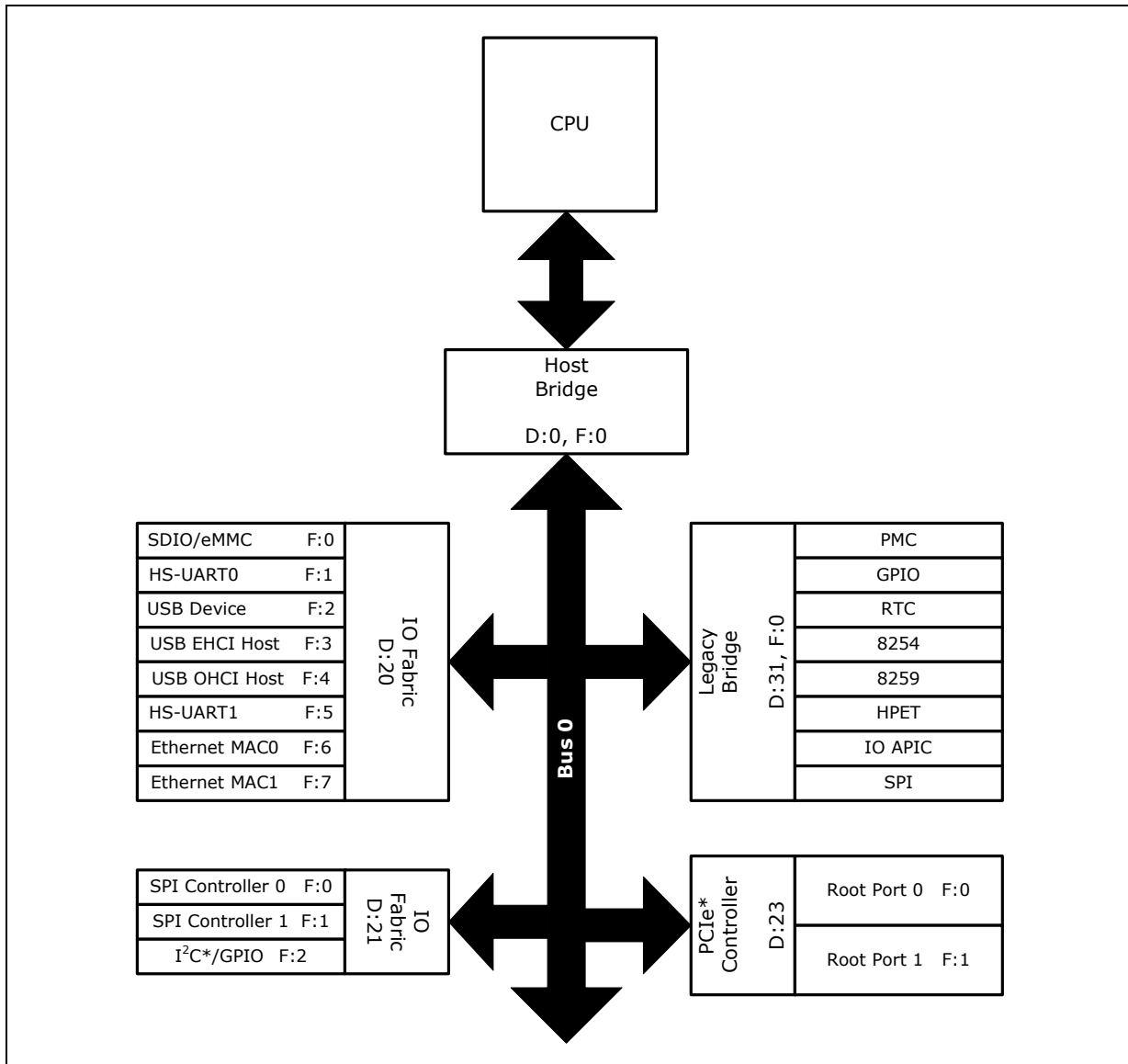
Figure 2. Intel® Quark SoC X1000 PCI View
