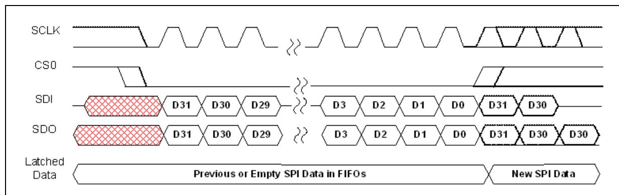
Figure 43. Generic SPI Waveform
