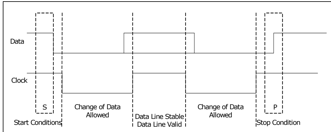
Figure 36. START and STOP Conditions
