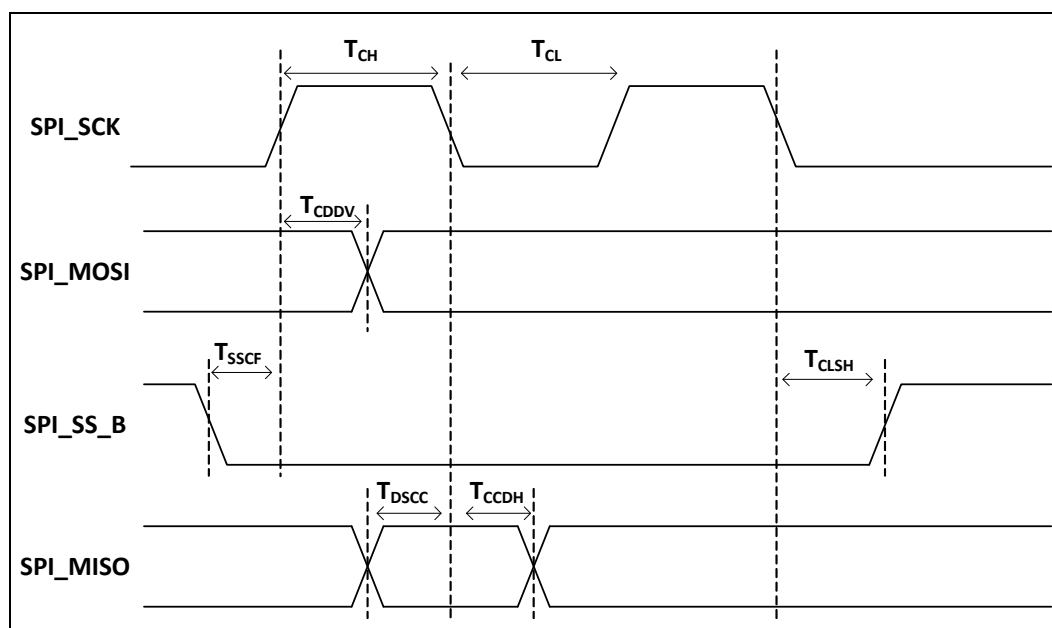
Figure 9. SPI Interface Timing
