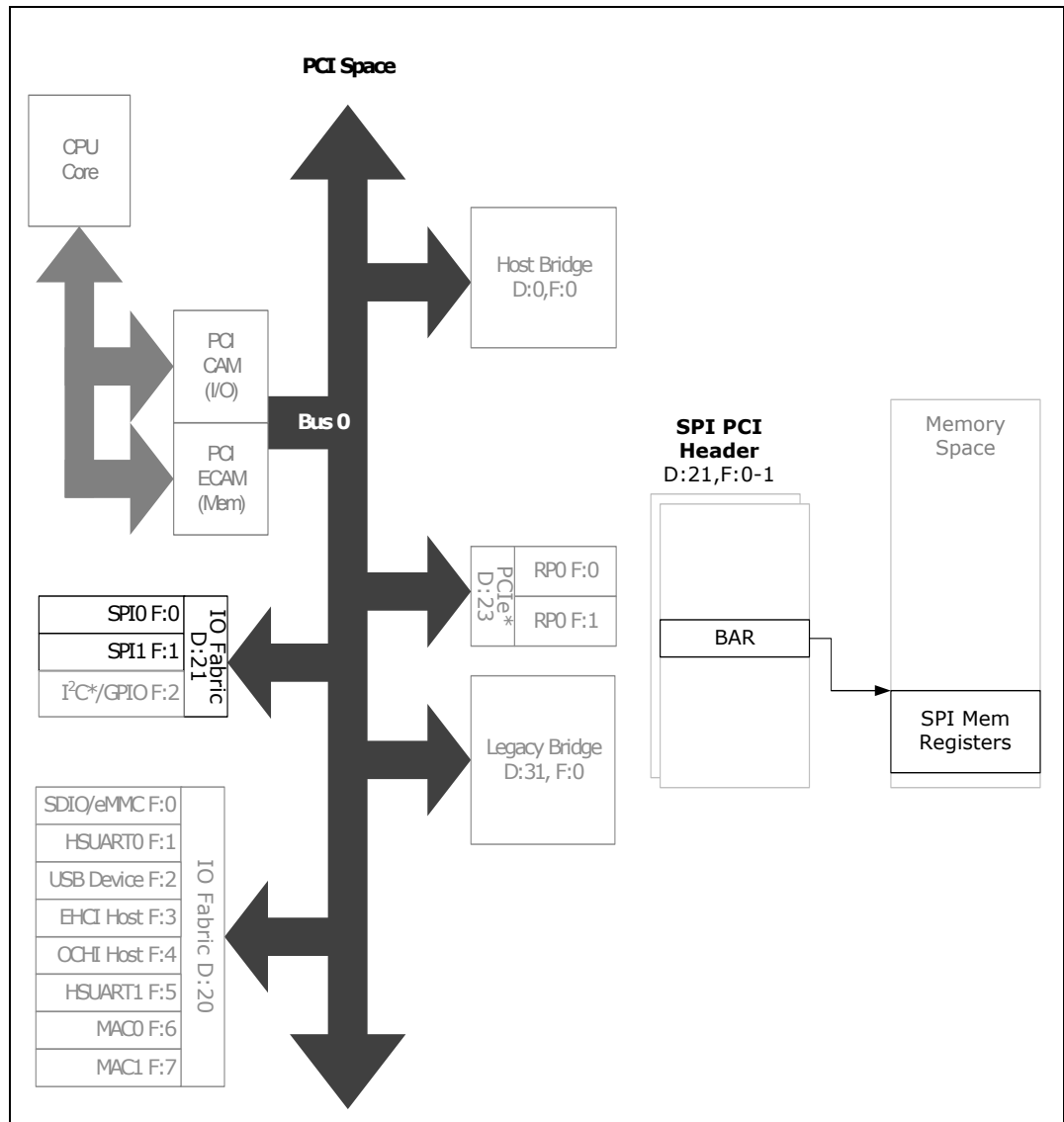
Figure 44. SPI Register Map
