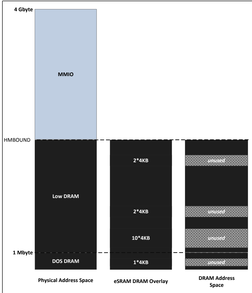
Figure 22. eSRAM 4KB Page Mapping
