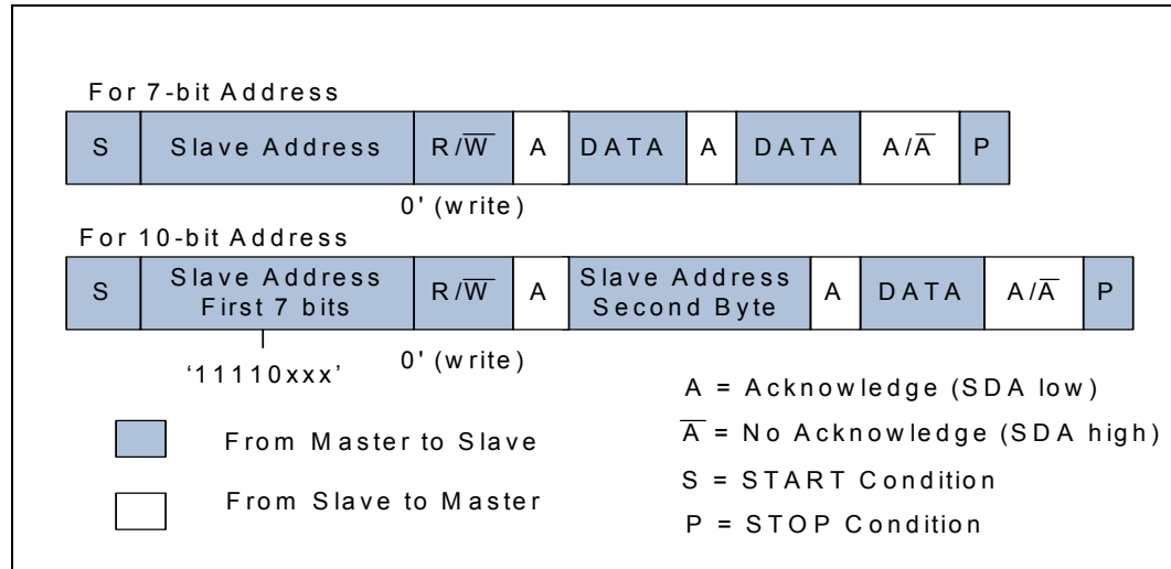
Figure 39. Master Transmitter Protocol
