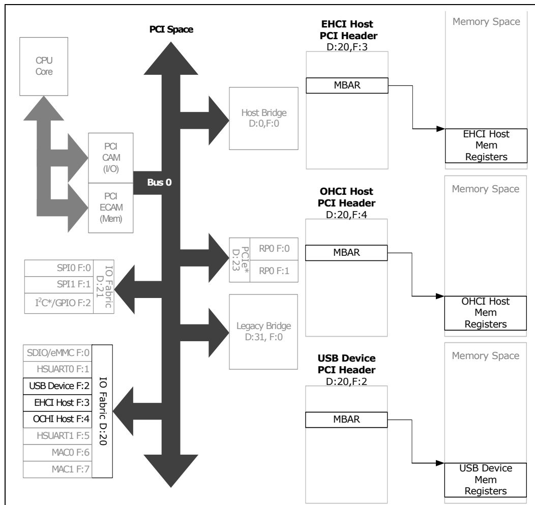
Figure 28. USB Register Map
