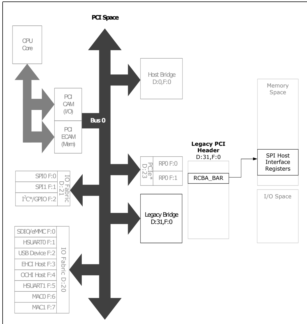
Figure 47. Legacy SPI Register Map
