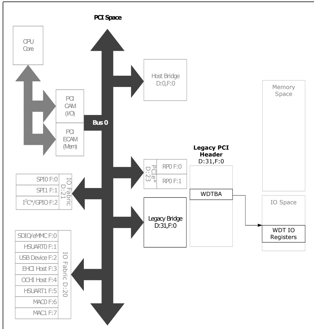
Figure 55. Watchdog Timer Register Map
