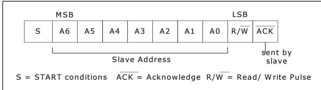
Figure 37. 7-Bit Address Format
