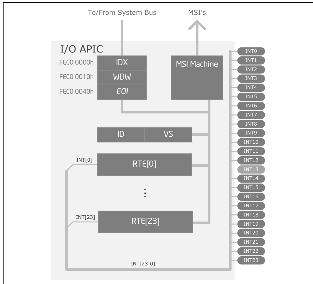
Figure 52. Detailed I/O APIC Block Diagram
