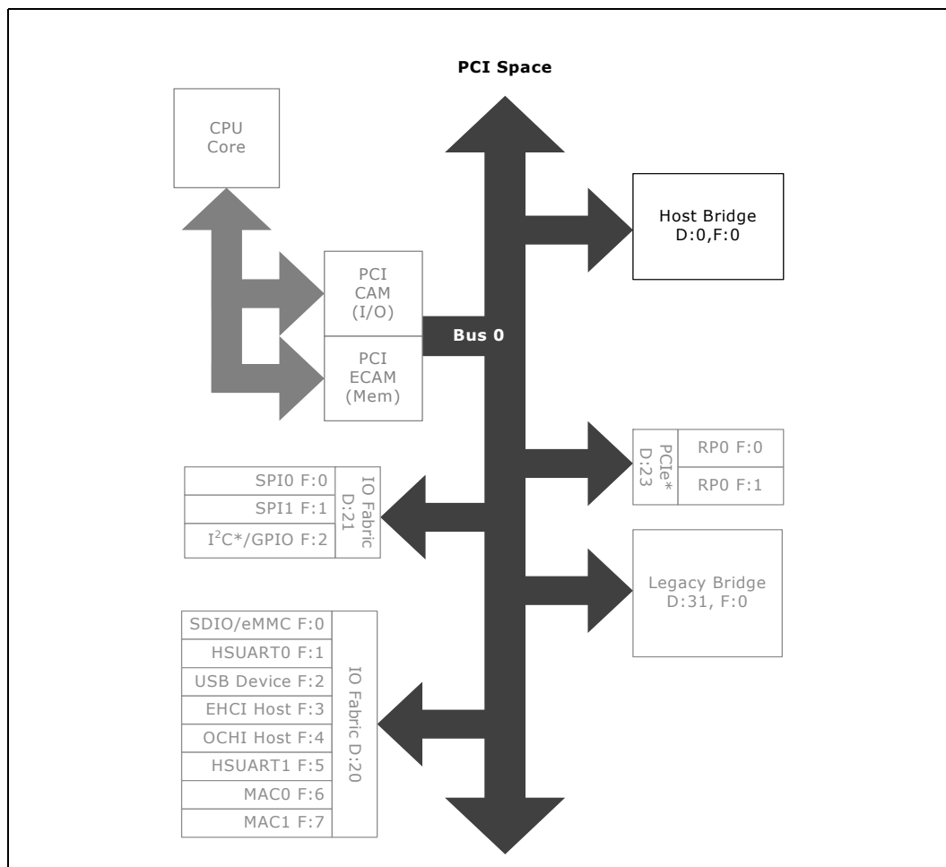
Figure 24. Intel® Quark SoC X1000 Host Bridge Register Map
