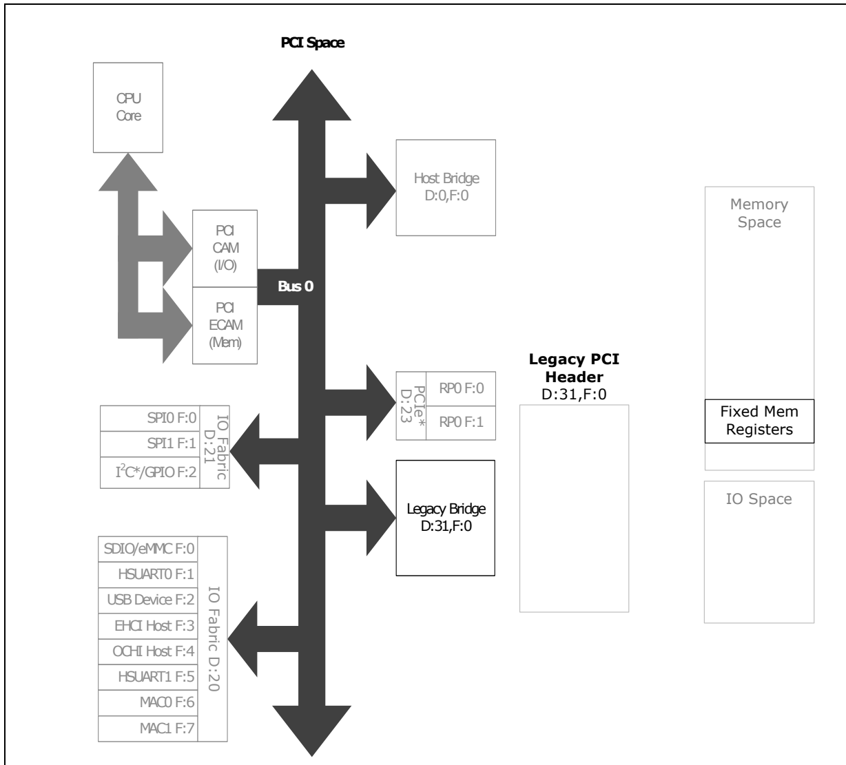
Figure 49. HPET Register Map
