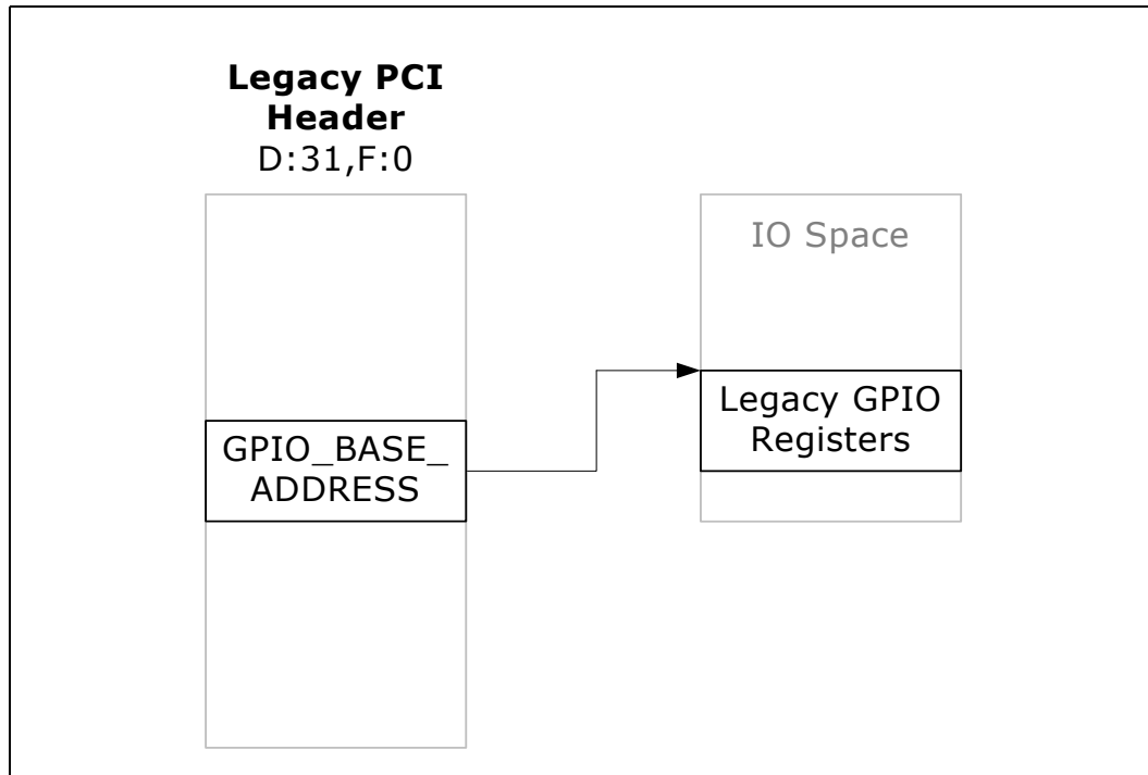
Figure 46. Legacy GPIO Register Map
