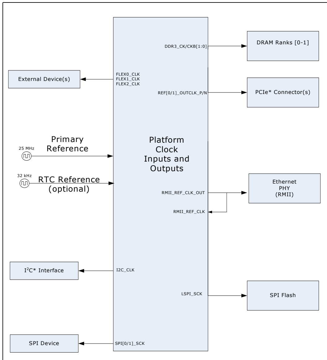
Figure 18. SoC Platform Clocking
