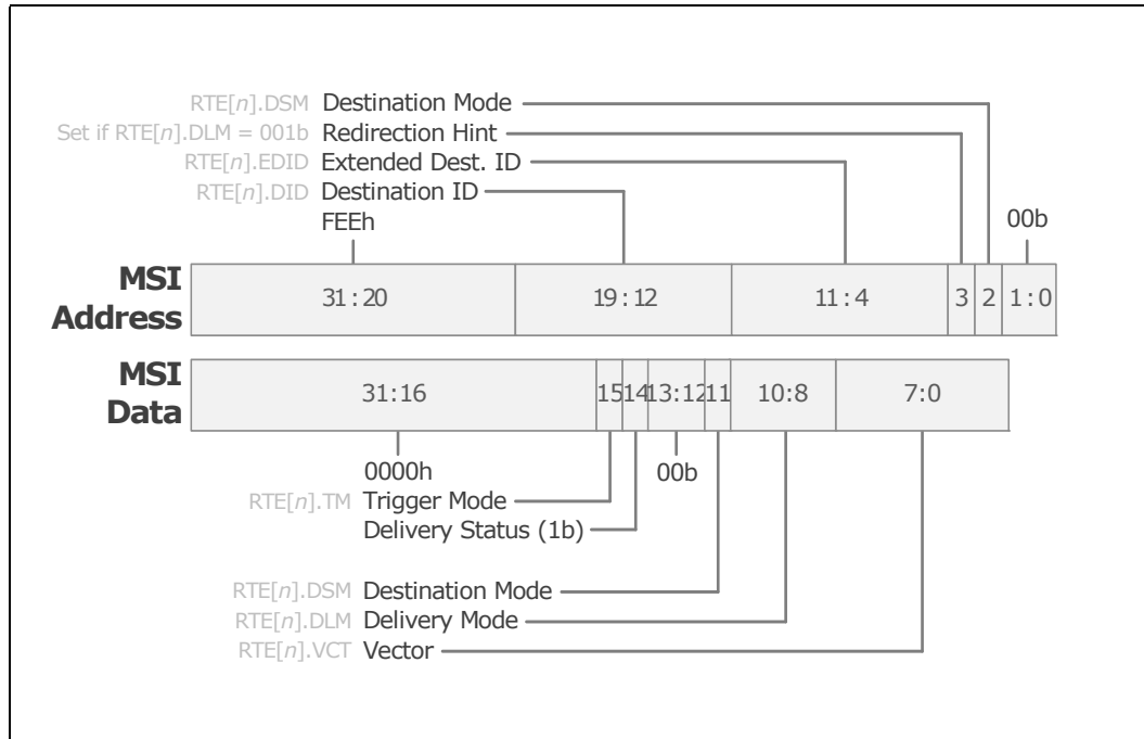
Figure 53. MSI Address and Data
