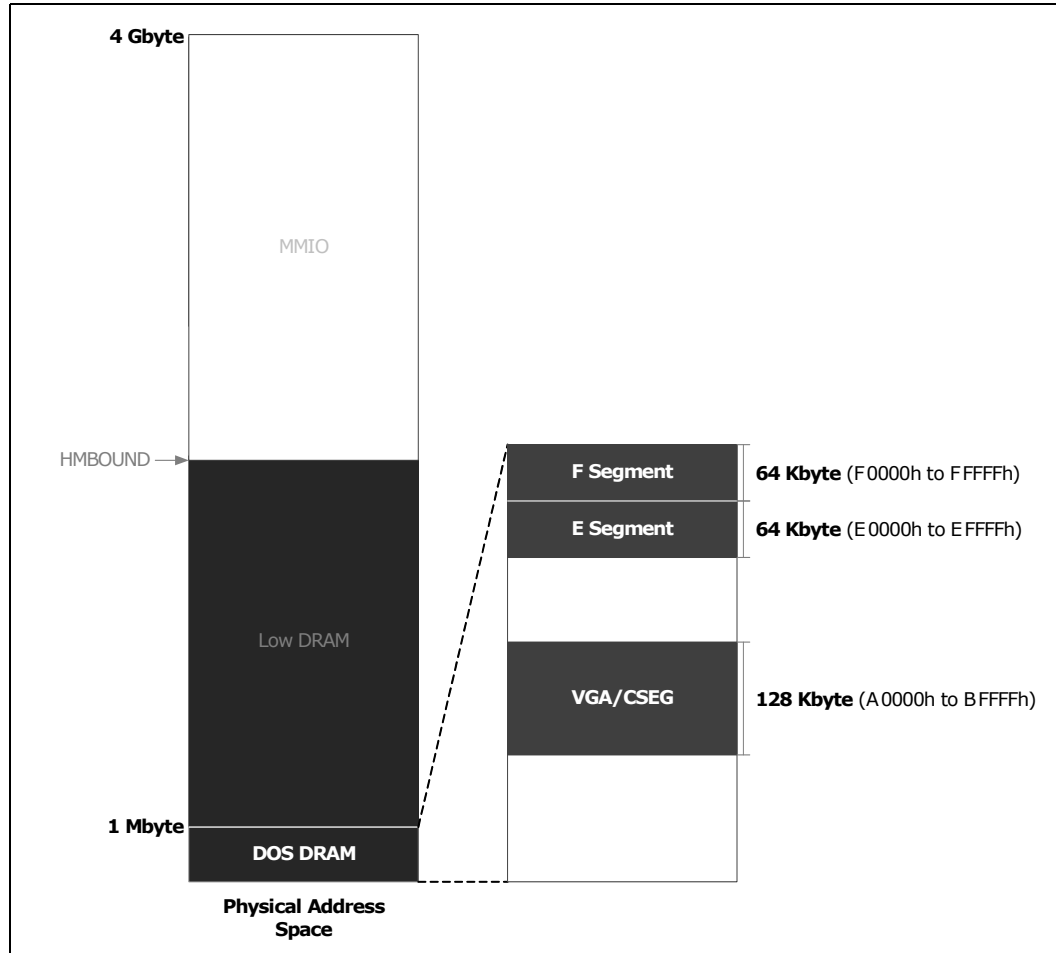
Figure 14. Physical Address Space - DOS DRAM
