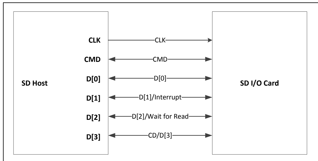
Figure 30. SDIO Card Bus Topology
