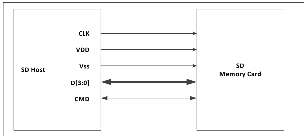
Figure 29. SD Memory Card Bus Topology
