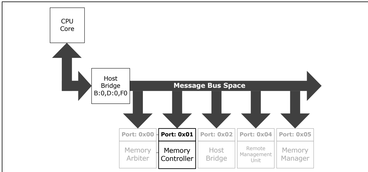
Figure 25. Register Map
