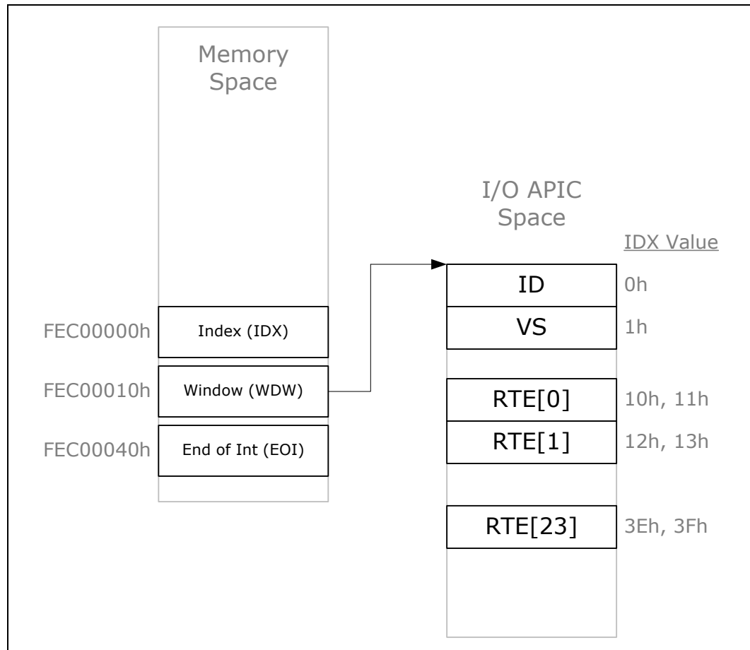
Figure 54. I/O APIC Register Map
