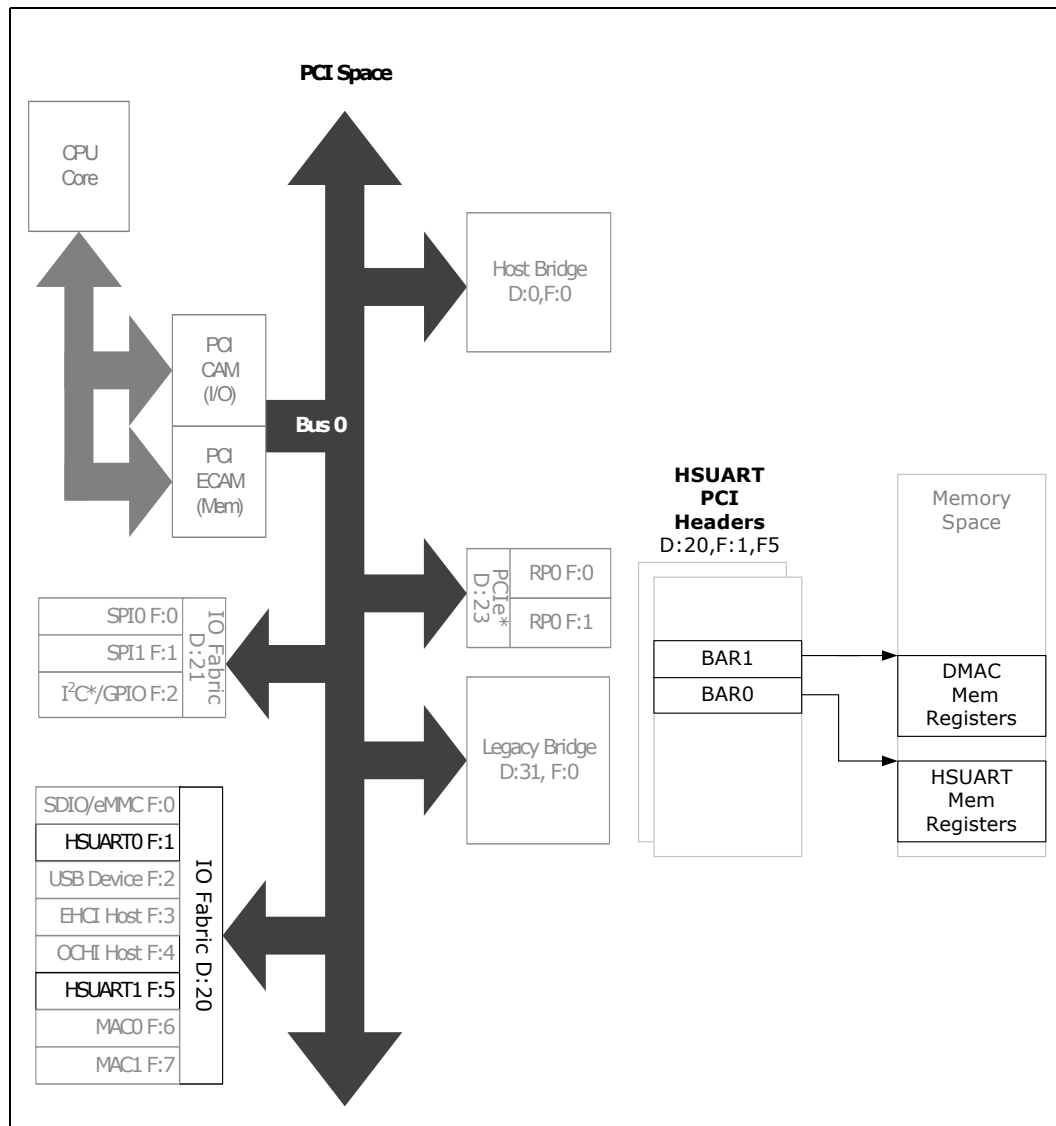
Figure 34. HSUART Register Map
