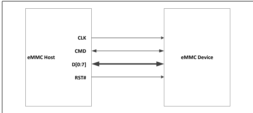
Figure 31. eMMC Interface
