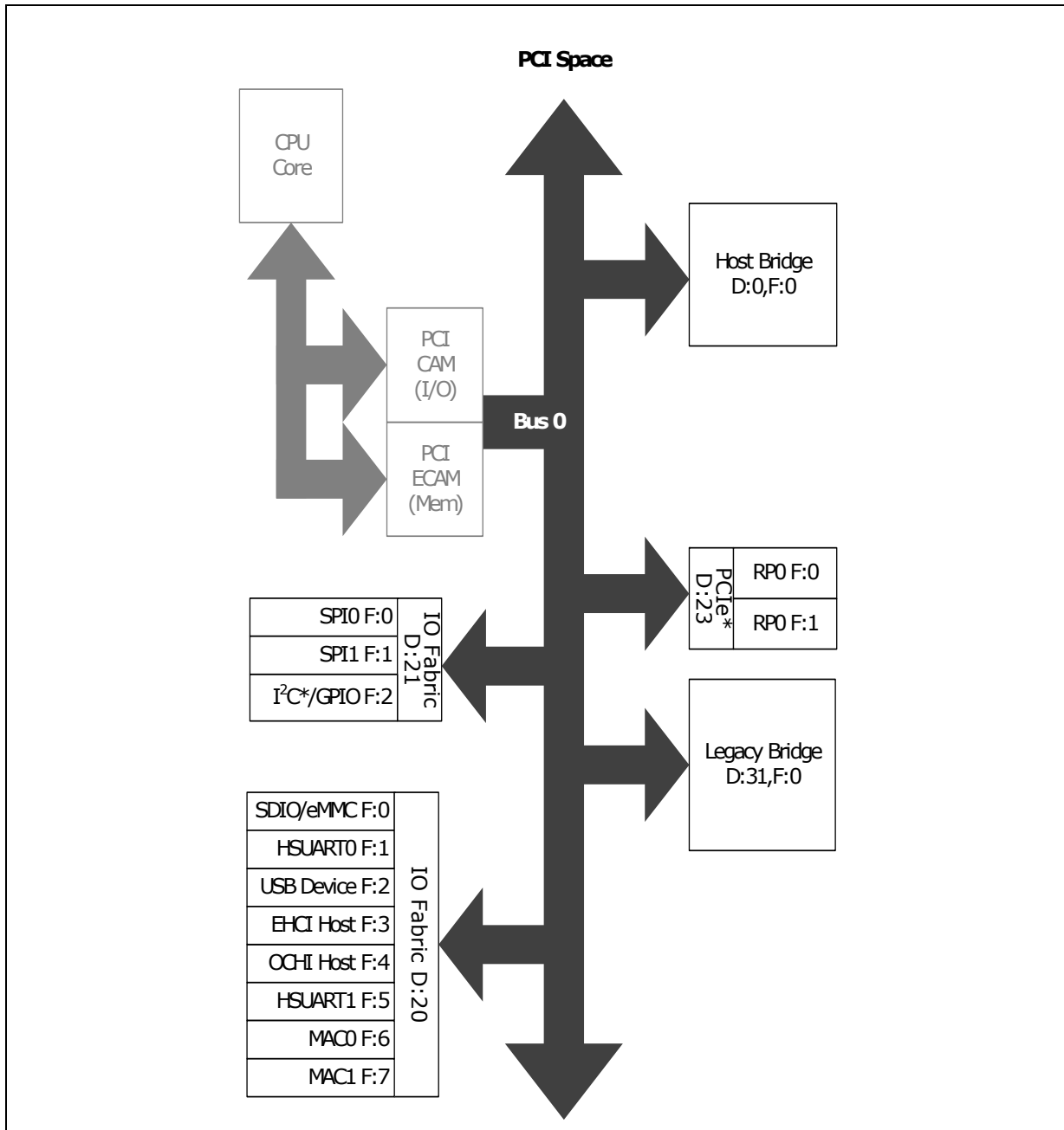
Figure 16. Bus 0 PCI Devices and Functions
