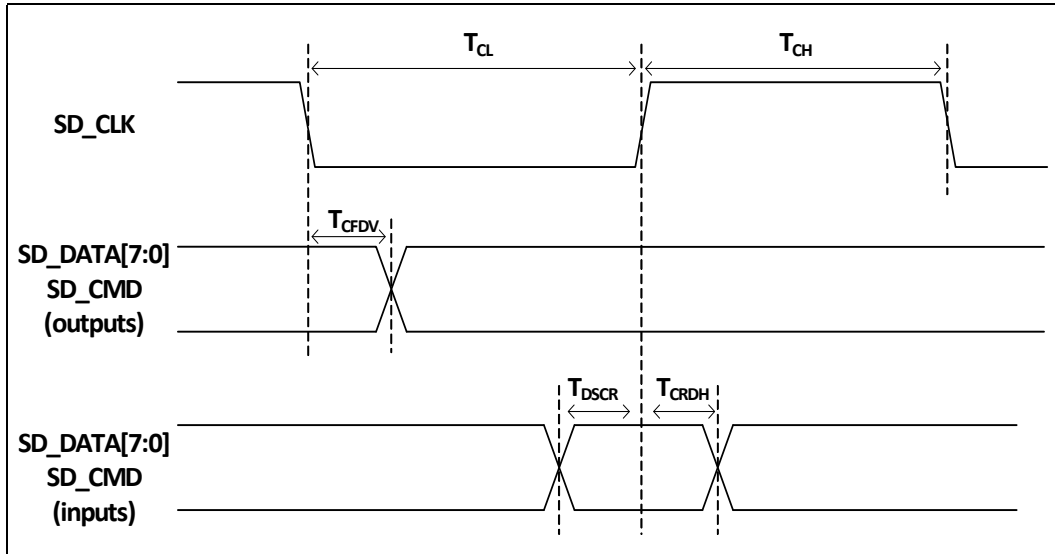
Figure 10. SDIO Interface Timing
