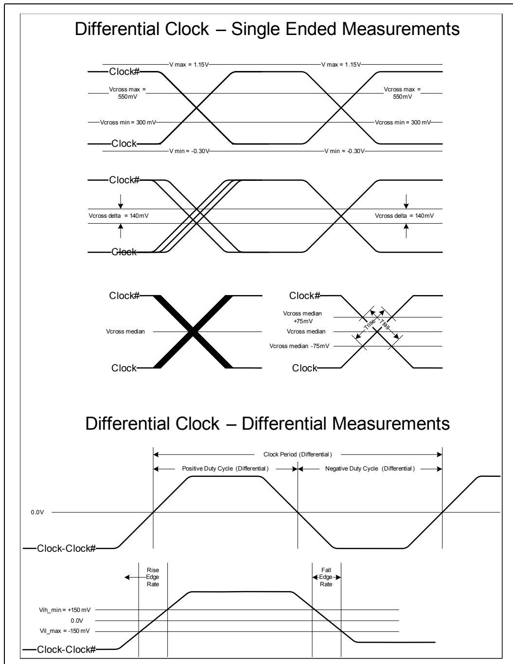
Figure 11. Measurement Points for Differential Clocks 1
