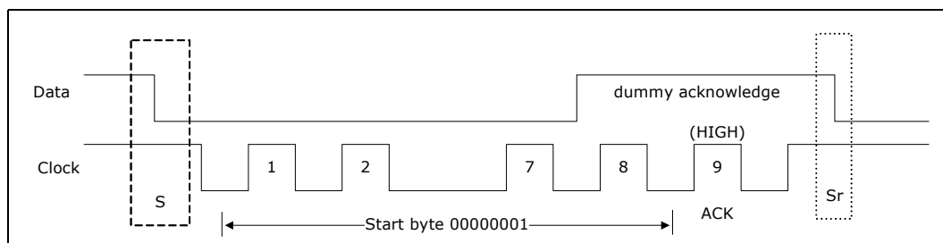
Figure 41. START Byte Transfer
