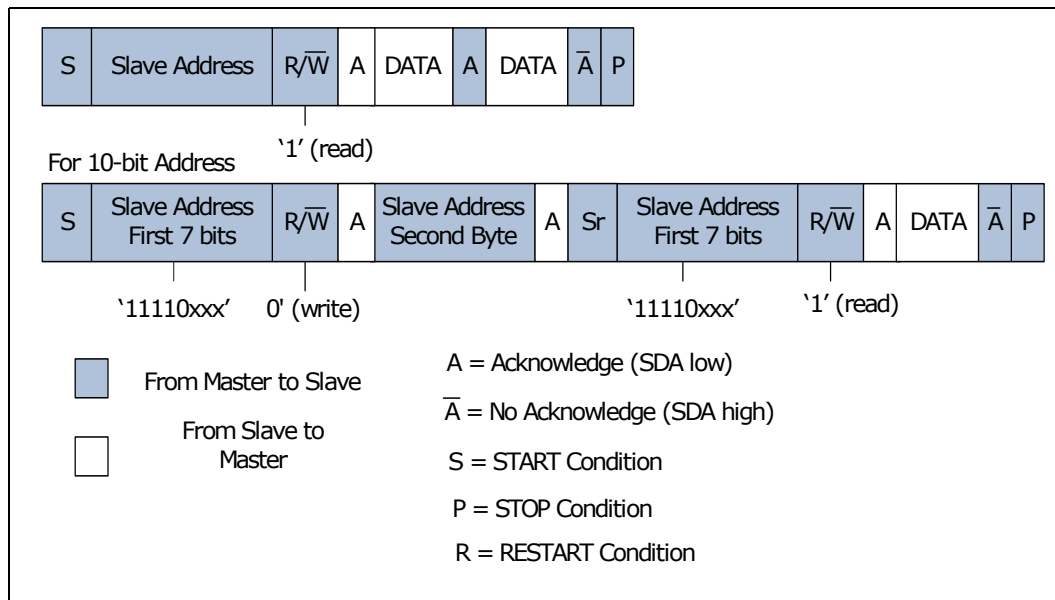
Figure 40. Master Receiver Protocol
