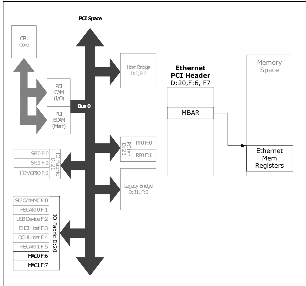
Figure 27. Ethernet Register Map
