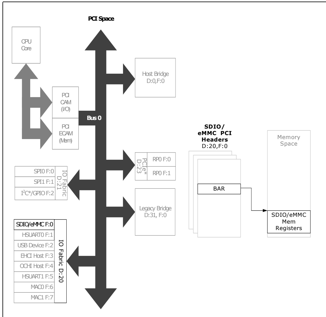
Figure 32. SDIO/SD/eMMC Register Map
