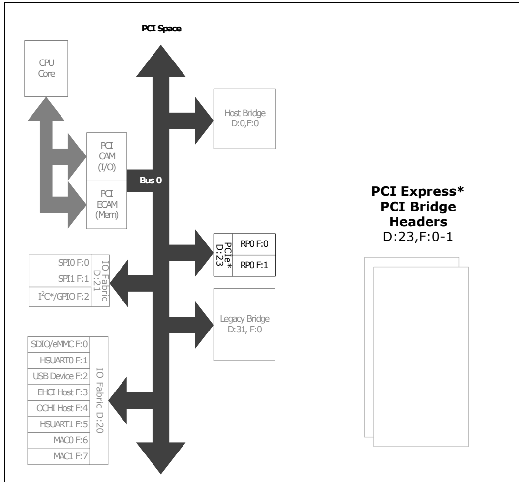
Figure 26. PCI Express Register Map
