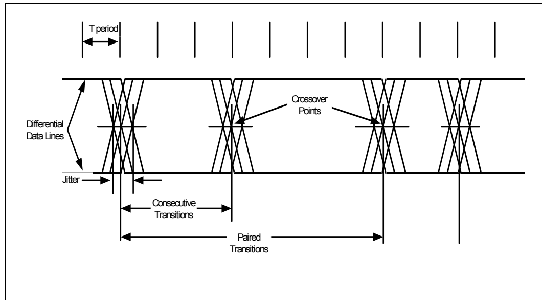
Figure 7. USB Jitter
