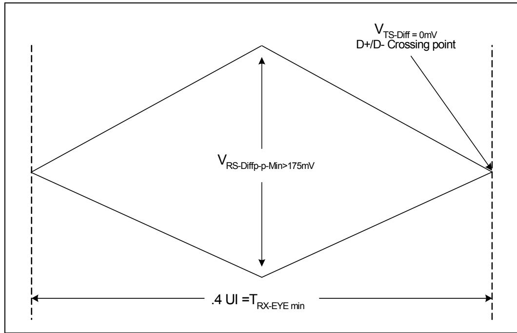
Figure 5. PCI Express Receiver Eye
