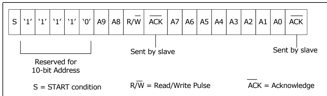
Figure 38. 10-bit Address Format
