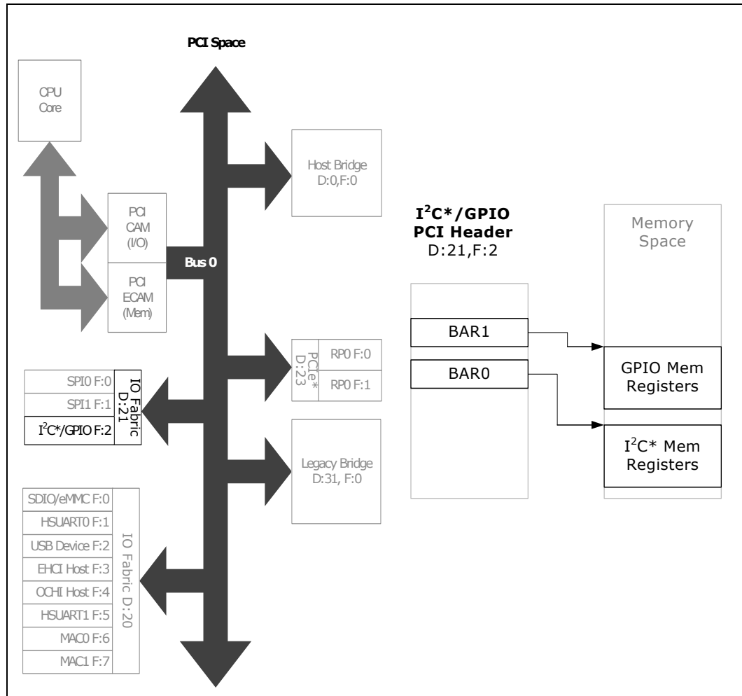
Figure 42. I 2 C*/GPIO Register Map
