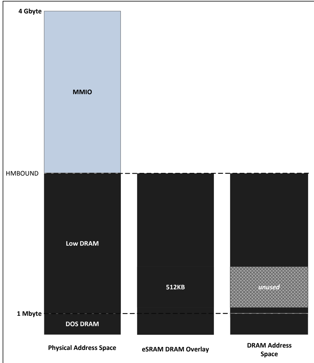
Figure 23. eSRAM 512KB Page Mapping
