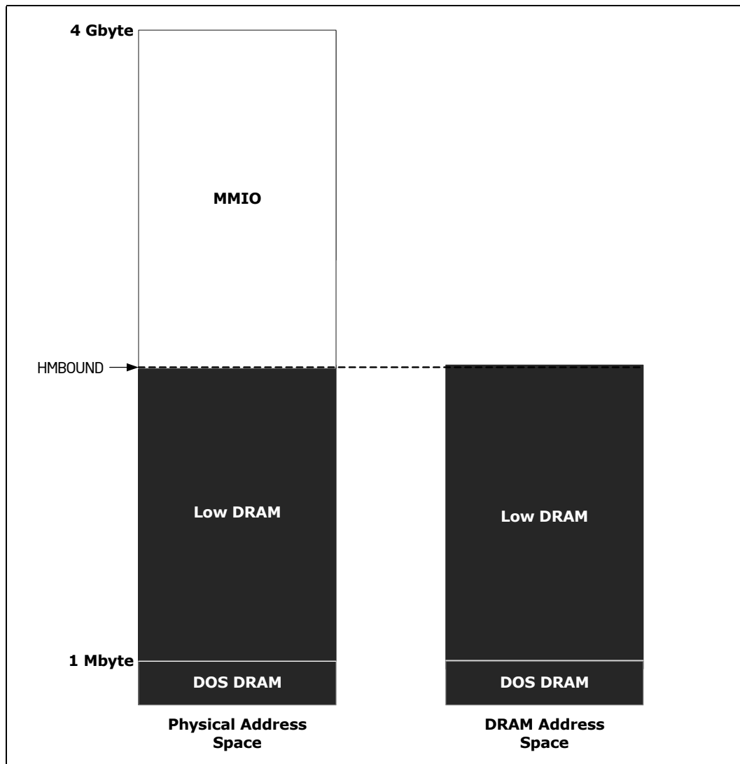
Figure 12. Physical Address Space - Low DRAM & MMIO
