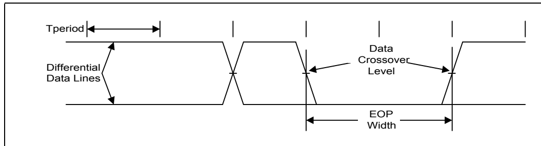
Figure 8. USB EOP Width
