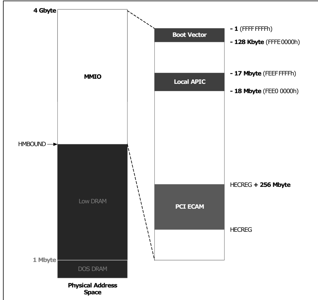
Figure 13. Physical Address Space - MMIO
