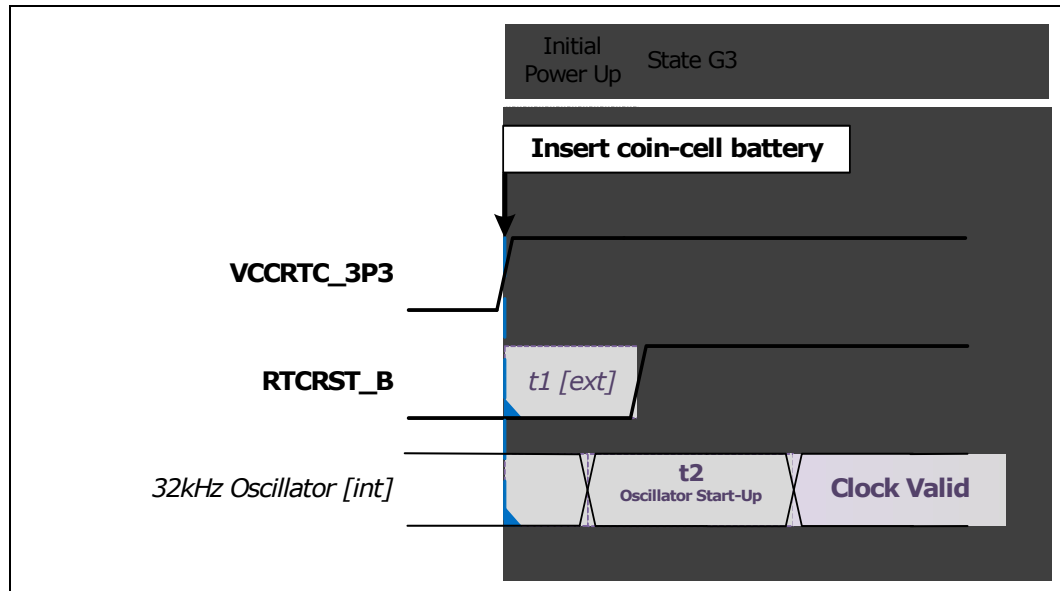
Figure 19. RTC Power Well Timing Diagrams
