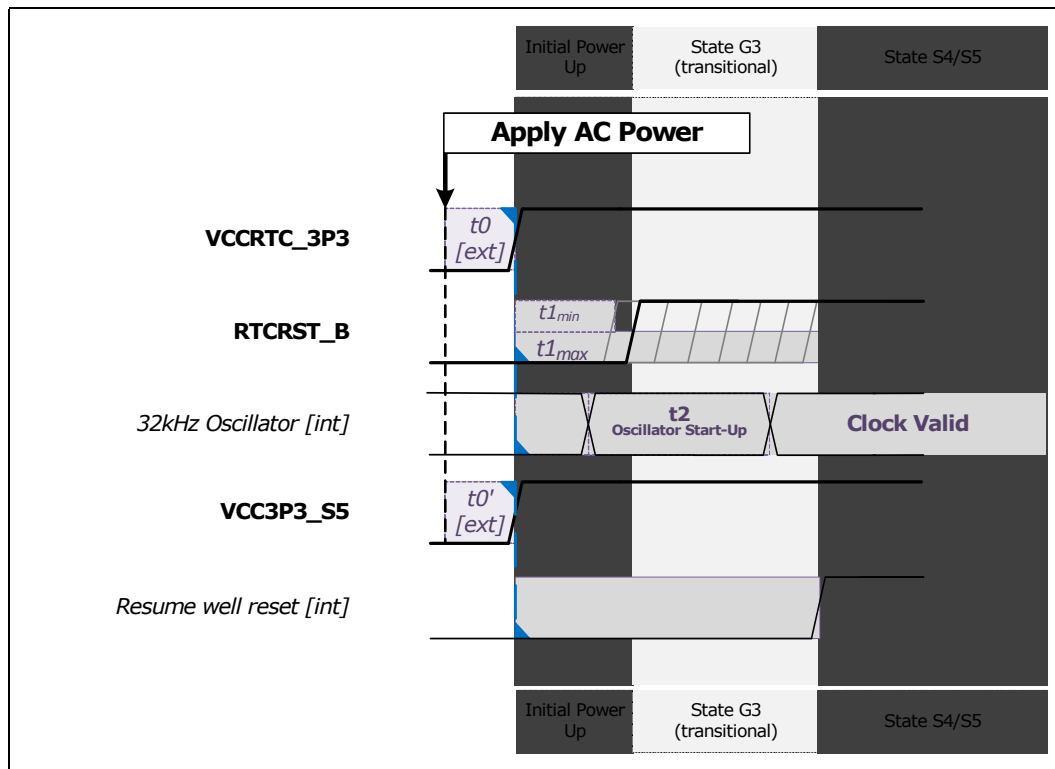
Figure 20. Power-Up Sequence without G2/G3
